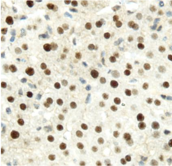
Immunohistochemistry of paraffin-embedded mouse liver using FNab10623(HNF4 antibody) at dilution of 1:100
