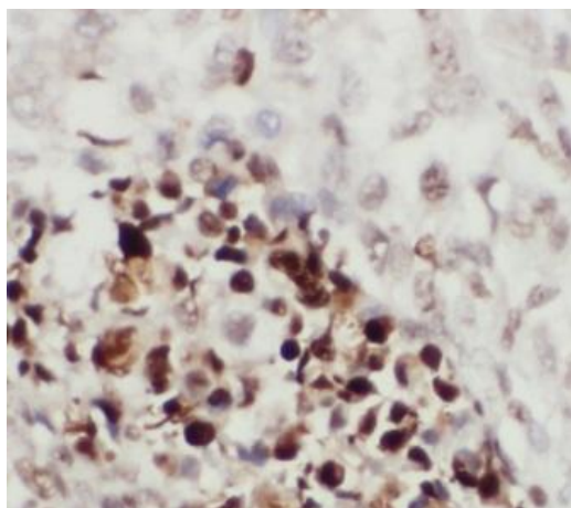
Immunohistochemistry of paraffin-embedded human lung cancer using FNab10329(ITCH antibody) at dilution of 1:100
