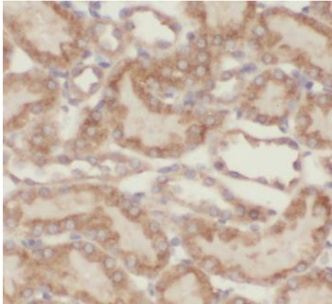
Immunohistochemistry of paraffin-embedded human kidney tissue slide using FNab09958(TOM40 Antibody) at dilution of 1:200
