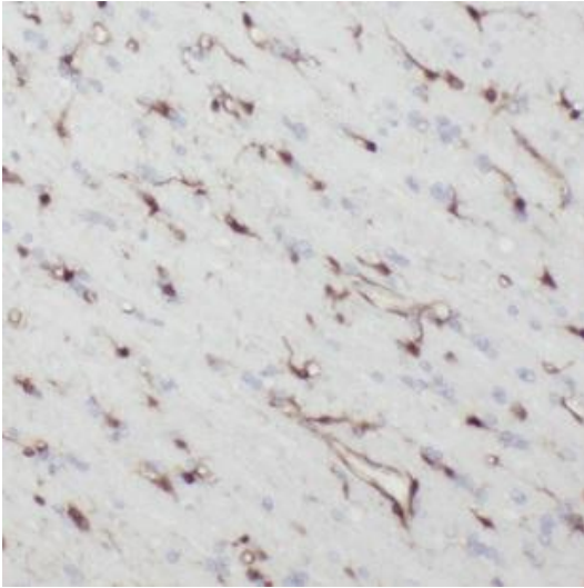
Immunohistochemistry of paraffin-embedded human oesophagus cancer using FNab05697(NEFH antibody) at dilution of 1:50
